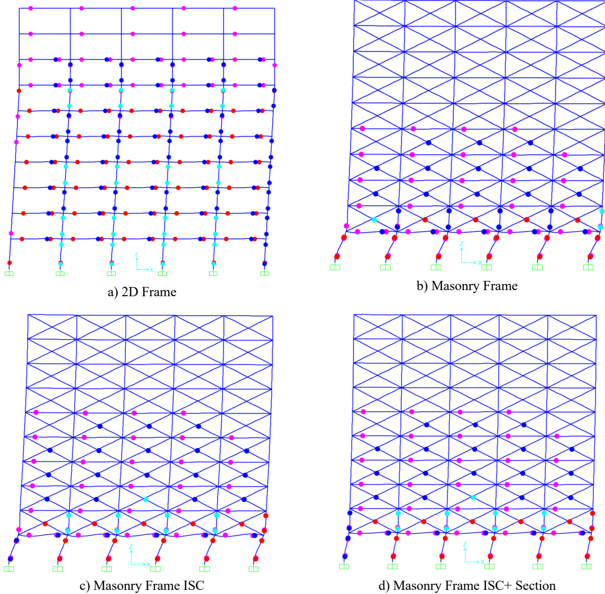
Figure 5: 10 story frame collapse during Earthquakes.
