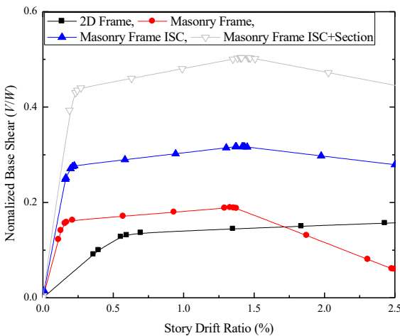
Figure 7: Push over curve 5 story frame.
