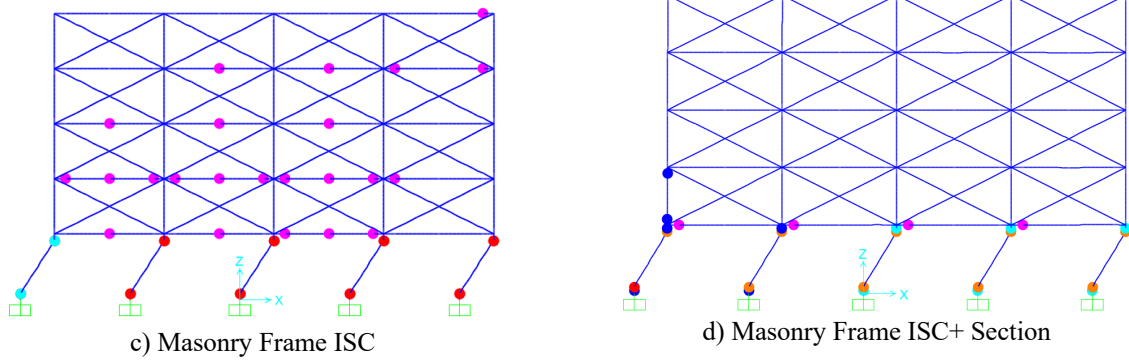
Figure 4: 5 story frame collapse during Earthquakes.
